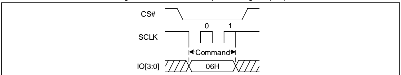
Figure 12 Write Enable Sequence Diagram (QPI)
