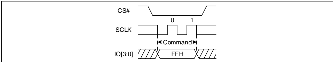
Figure 59 Disable QPI mode command Sequence Diagram
