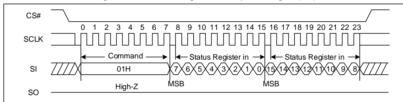
Figure 17. Write Status Register-1&2 Sequence Diagram (SPI)
