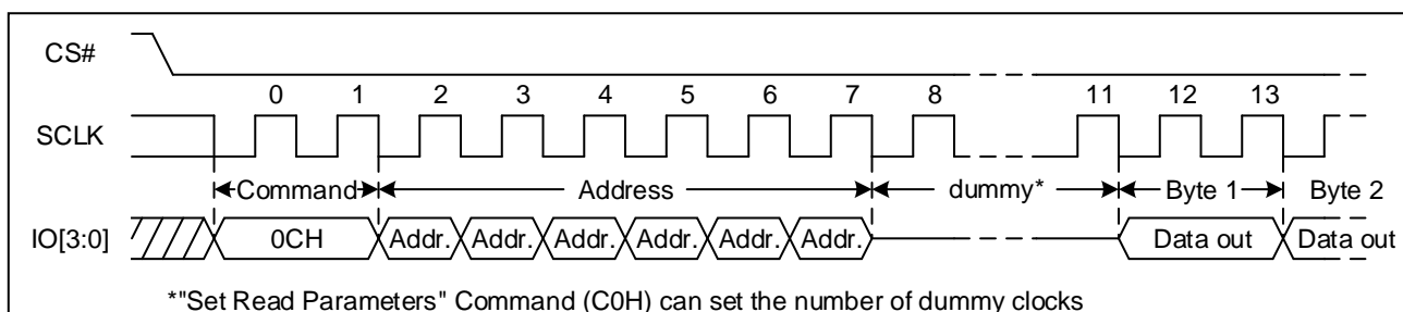
Figure 43. Burst Read with Wrap Sequence Diagram
