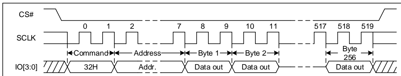
Figure 49 Quad Page Program Sequence Diagram (QPI)
