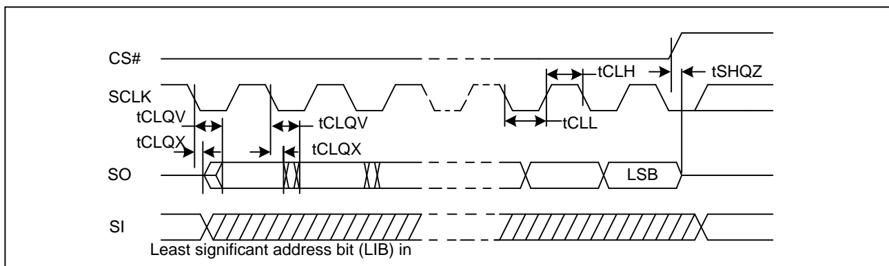
Figure 98. Output Timing
