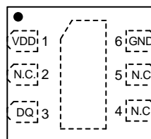
DFN Top View
