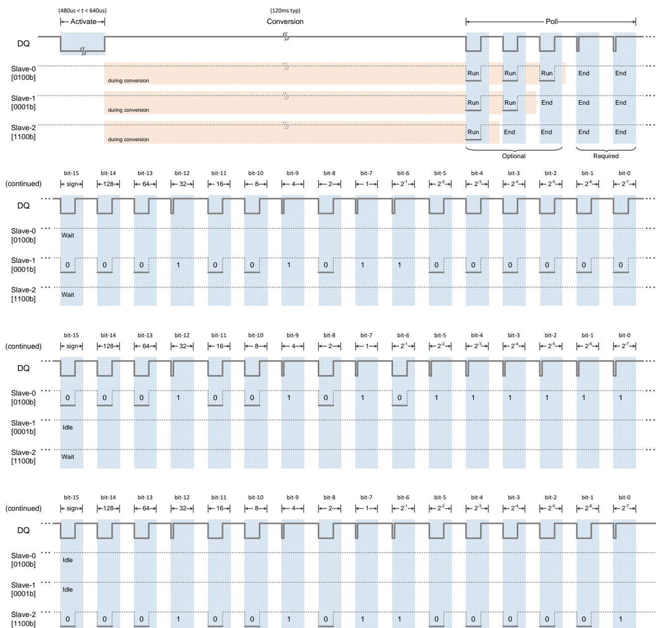
Figure 6. Signal Timing Diagram of Temperature Reading Process
