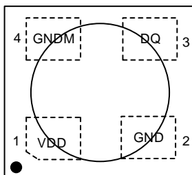
MCLGA Top View
