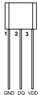
TO-92S Front View
