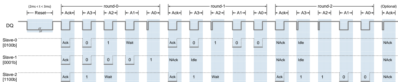
Figure 5. Signal Timing Diagram of the Search Process
